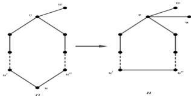
Fig. 1 Transformation of G into H .
